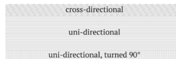
Combination Construction
